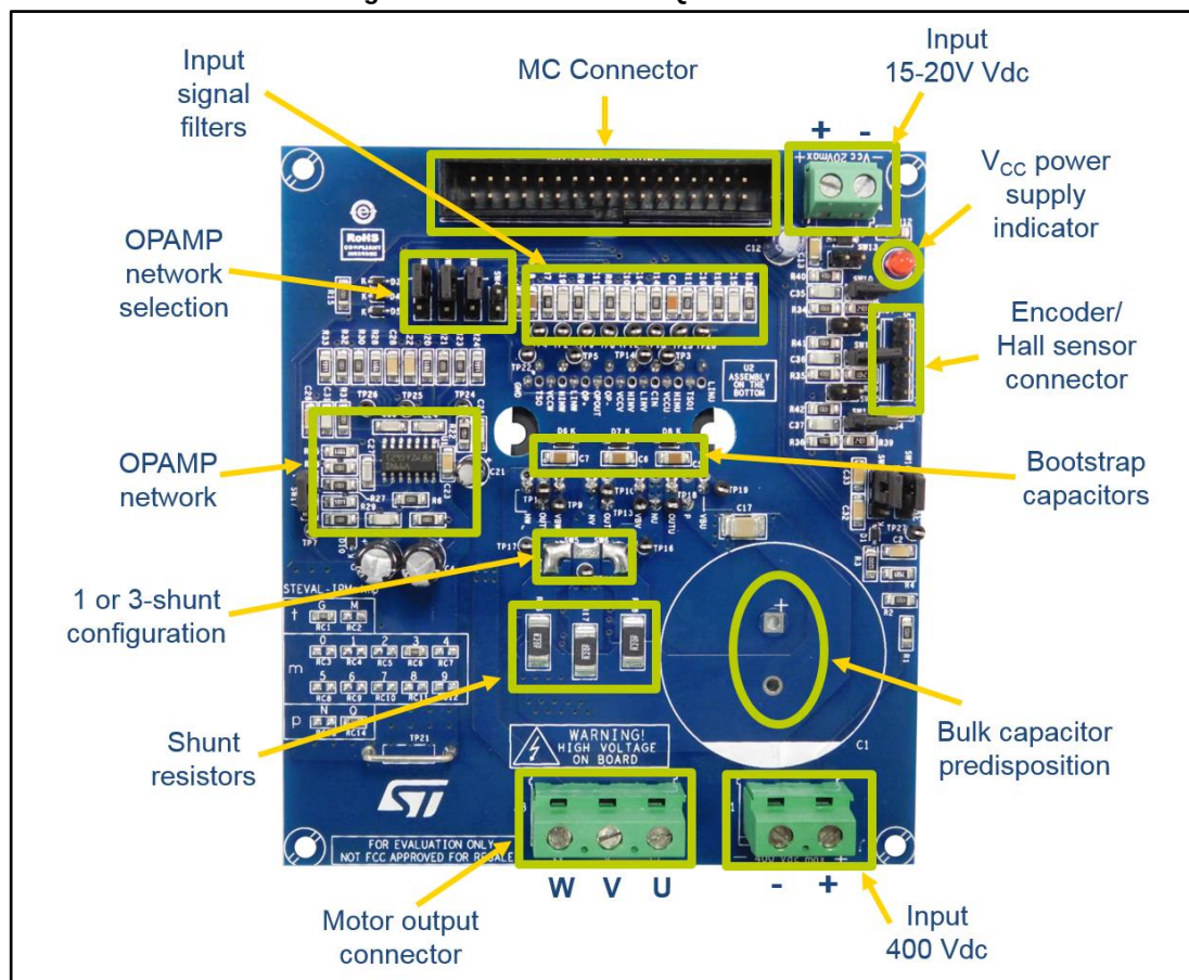
Figure 8: STEVAL-IPMNG5Q architecture
