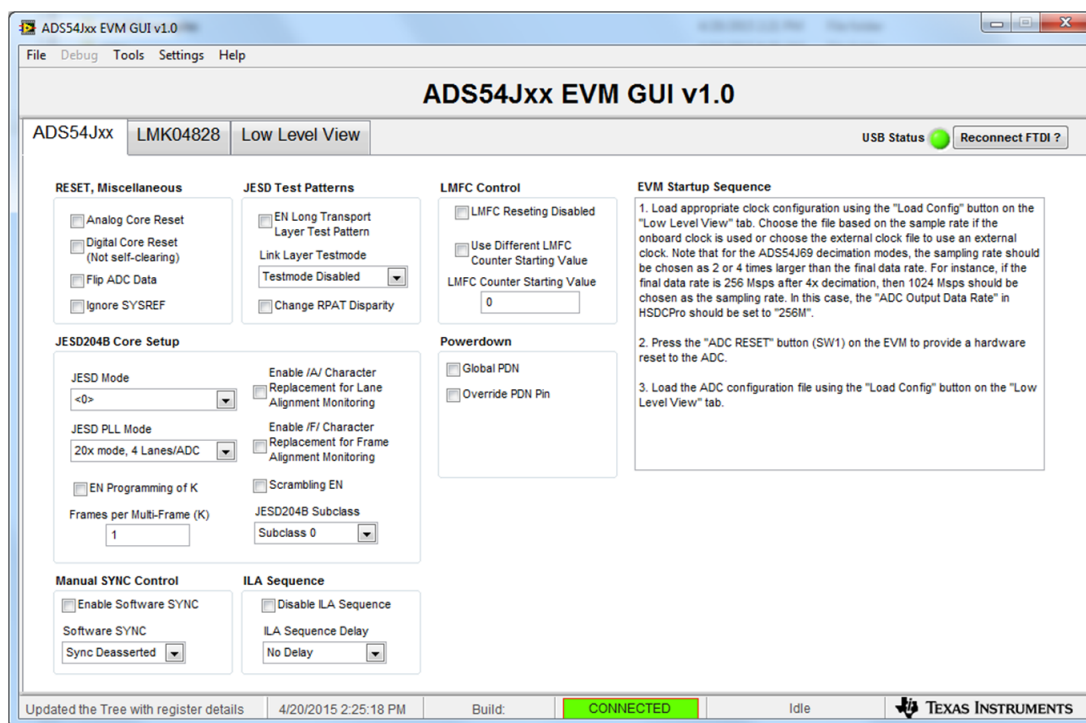
Figure 6. ADS54Jxx GUI
