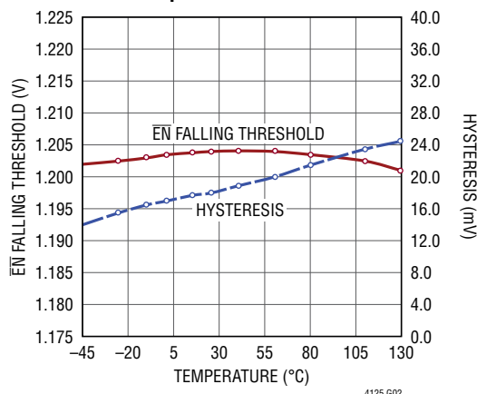
EN Threshold Over Temperature
