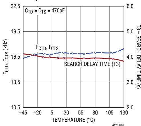
C_{TS} , C_{TD} Pin Frequency and Search Delay Time Over Temperature
