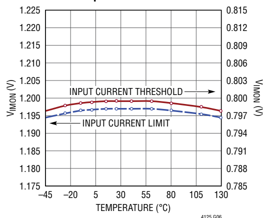
Input Current Threshold and Limit Over Temperature
