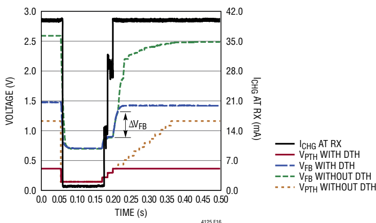
Figure 16. V_{FB} Voltage Stepping During A Sweep with LTC4120 in Trickle Charge CC Mode as the Receiver Circuit at 10mm Spacing
