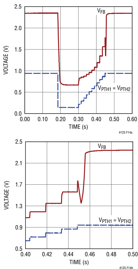
Figure 14. FB, PTH1 and PTH2 Pins Voltage Stepping During a Sweep with C_{TS} = 4.7\text{nF}
