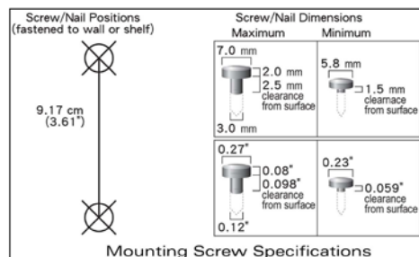
Figure 1: PoE Midspan mounting instructions
