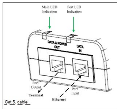
Figure 3: PoE Midspan Ports
