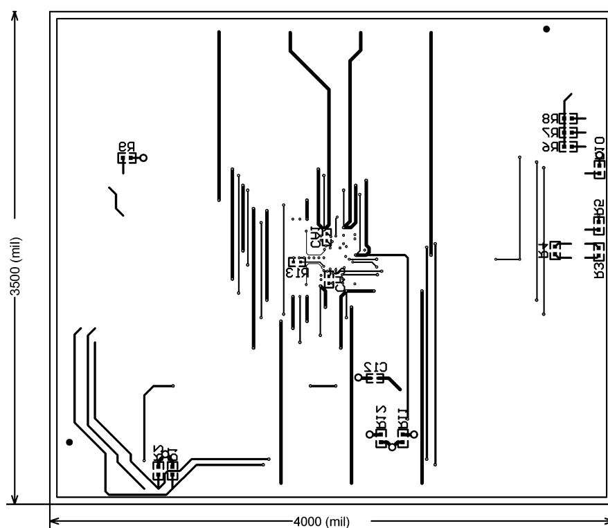
Figure 7. Bottom Layer
