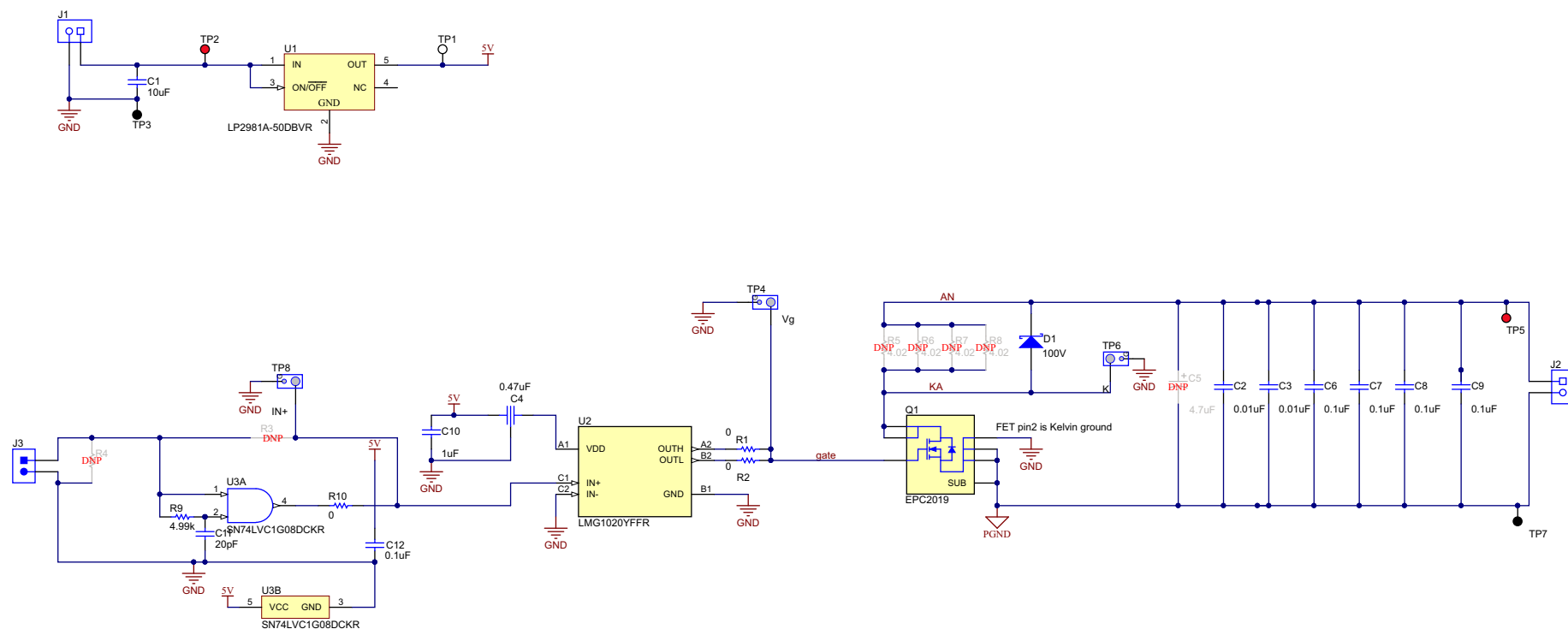
Figure 4. Power Stage Schematic (DNP = Do Not Place, Not Present On Board)
