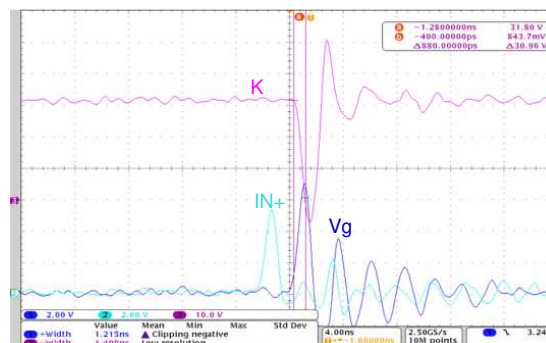
Figure 12. 1.2-ns Gate Pulse Yielding 1.5 ns, 30 V into 1-Ω Pulse (500-MHz Scope)
