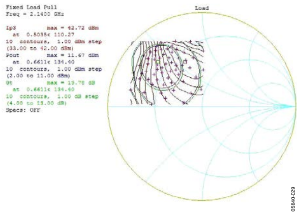
Figure 37. Load-Pull Contours, 2140 MHz
