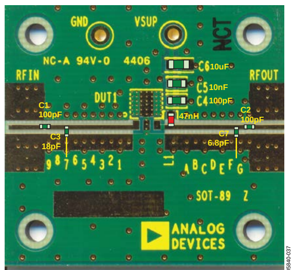
Figure 43. Evaluation Board Layout and Component Placement 450 MHz to 500 MHz Operation
