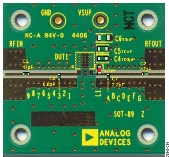
Figure 44. Evaluation Board Layout and Component Placement 800 MHz to 960 MHz Operation
