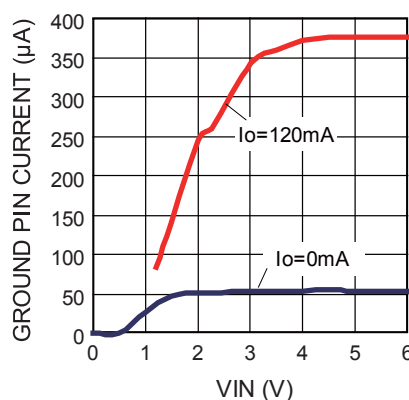
Ground Pin Current vs. V_{IN}
