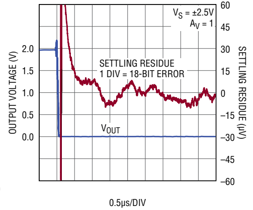
18-Bit Settling Time to 2V P-P Output Step
