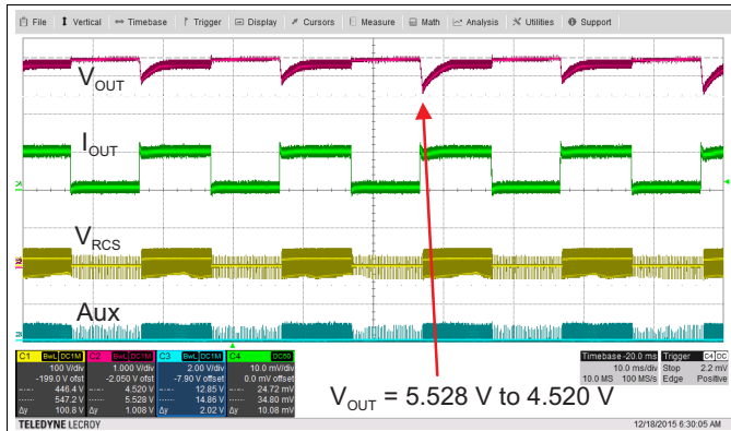
Figure 13. V_{IN} = 85 V RMS
