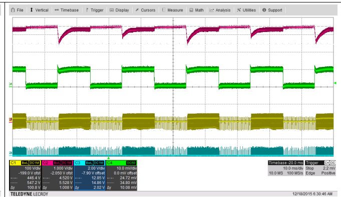
Figure 14. V_{IN} = 115 V RMS
