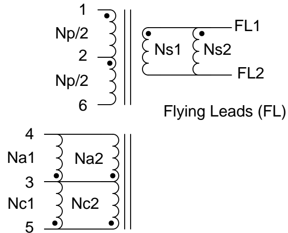
Figure 24. Transformer Schematic
