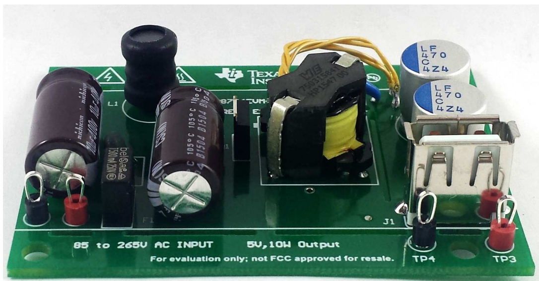
Figure 1. UCC28704EVM-724
