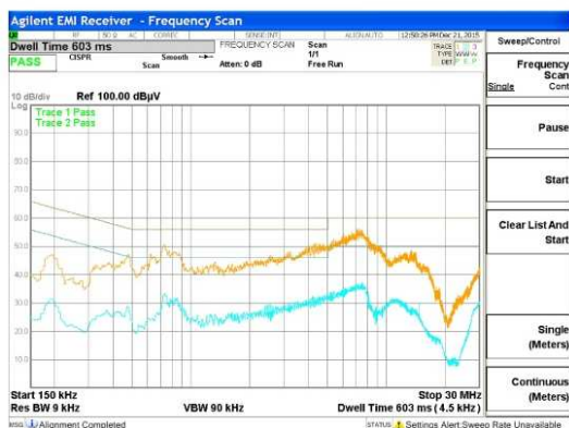
Figure 22. VIN = 115 V RMS , Load = 2.5 Ω
