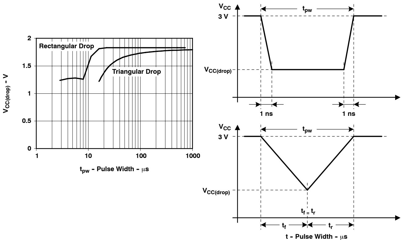
Figure 10. V_{CC(drop)} With a Square Voltage Drop and a Triangular Voltage Drop to Generate an SVS Signal
