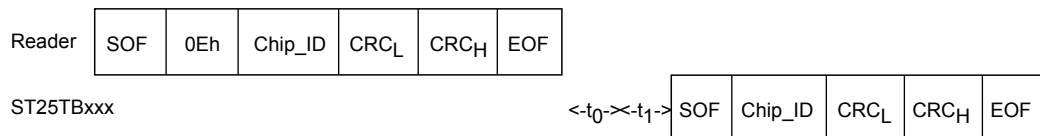
Figure 29. Select frame exchange between reader and ST25TB02K
