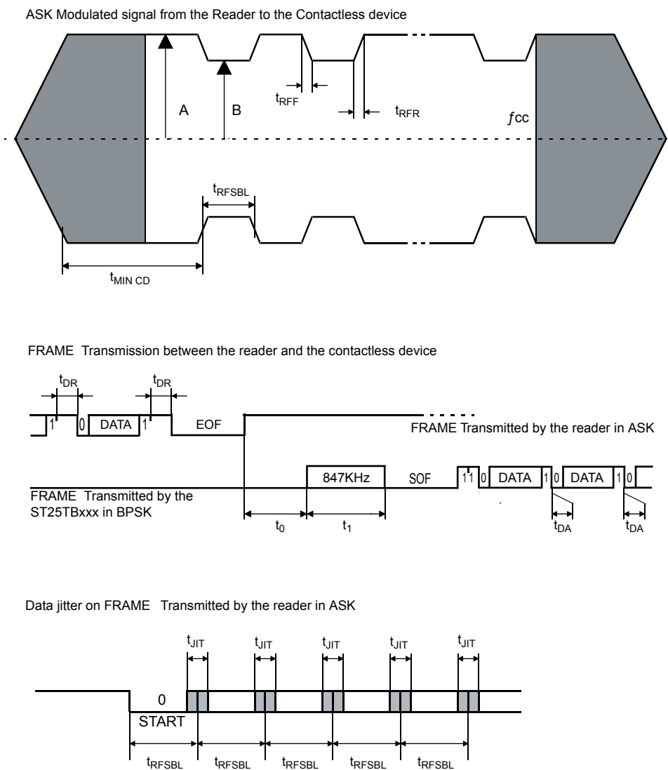
Figure 46. ST25TB02K synchronous timing, transmit and receive
