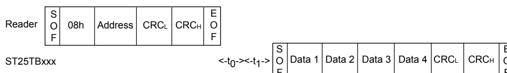
Figure 38. Read_block frame exchange between reader and ST25TB02K
