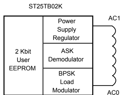
Figure 1. Logic diagram
