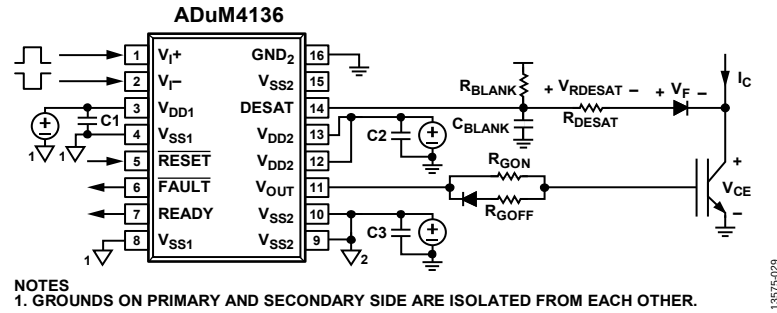
Figure 29. Typical Application Schematic
