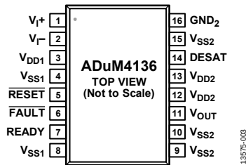
Figure 3. Pin Configuration
