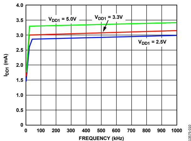
Figure 10. I_{DD1} Current vs. Frequency, Duty = 50%, V_{I+} = V_{DD1}
