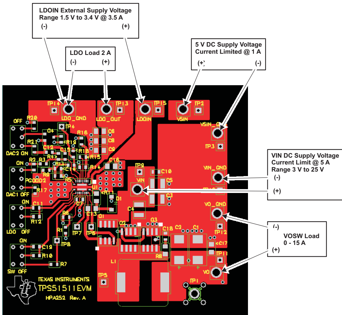
Figure 7. Test Setup
