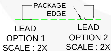
Figure 18. 10-Lead, Quad Ultrathin Molded Leadless Package (UMLP)
