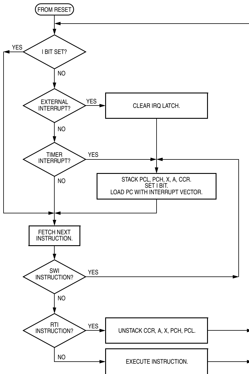
Figure 5-3. Interrupt Flowchart
