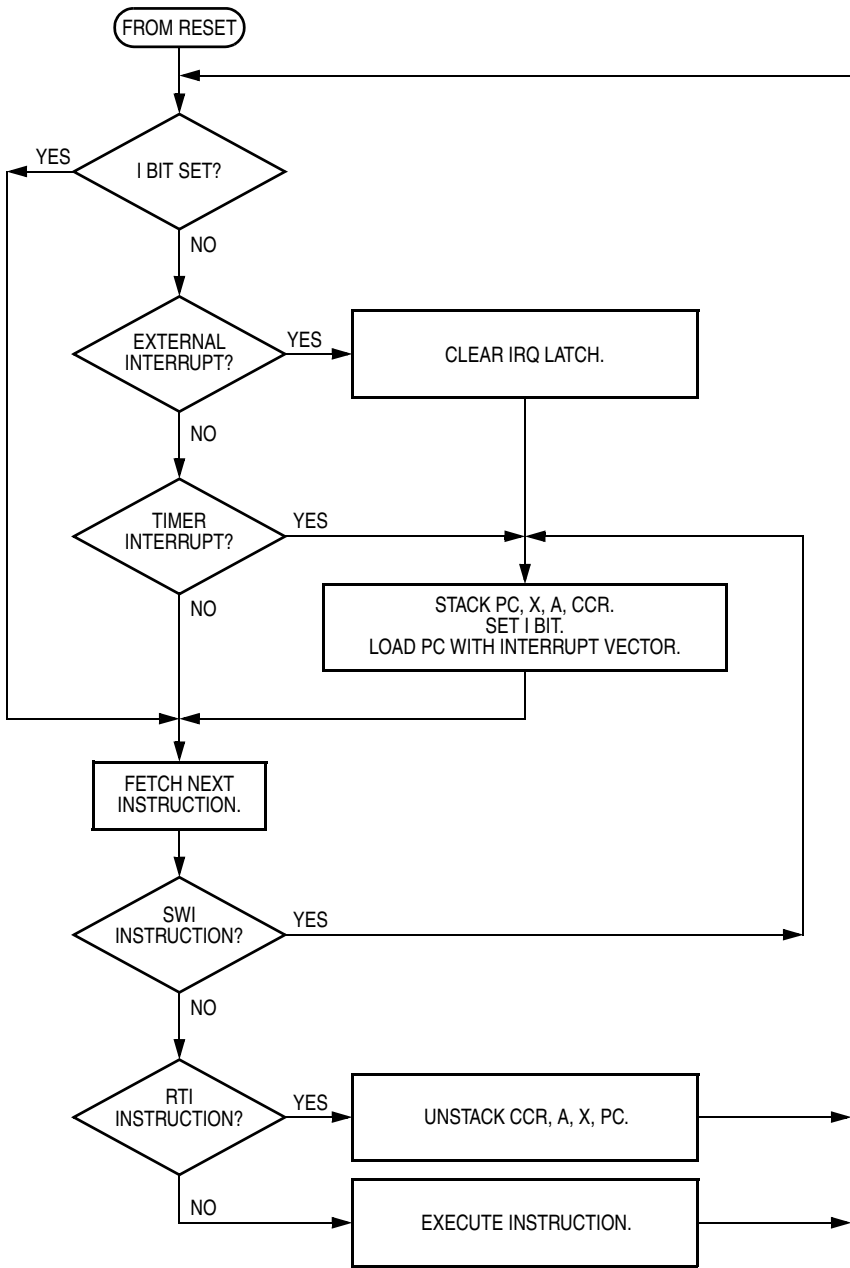
Figure 8-7. Interrupt Flowchart
