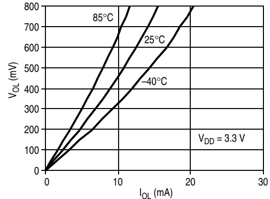
Figure 10-3. PA4–PA7 Typical Low-Side Driver Characteristics
