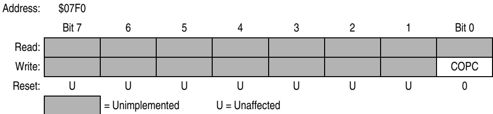
Figure 3-1. COP Register (COPR)
