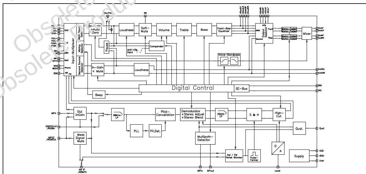
Figure 2. BLOCK DIAGRAM
