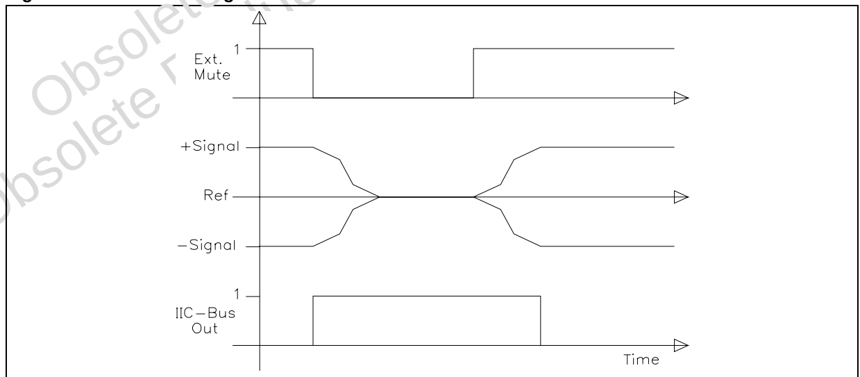
Figure 9. Softmute-Timing
