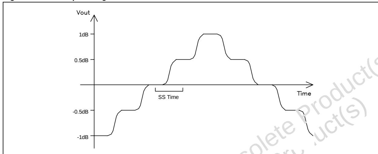
Figure 10. SoftStep-Timing
