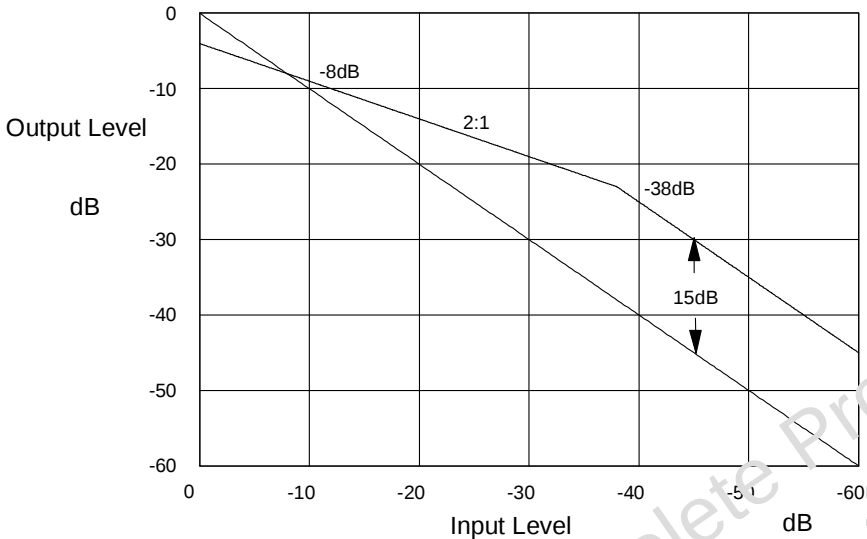
Figure 22. Comander Characteristic
