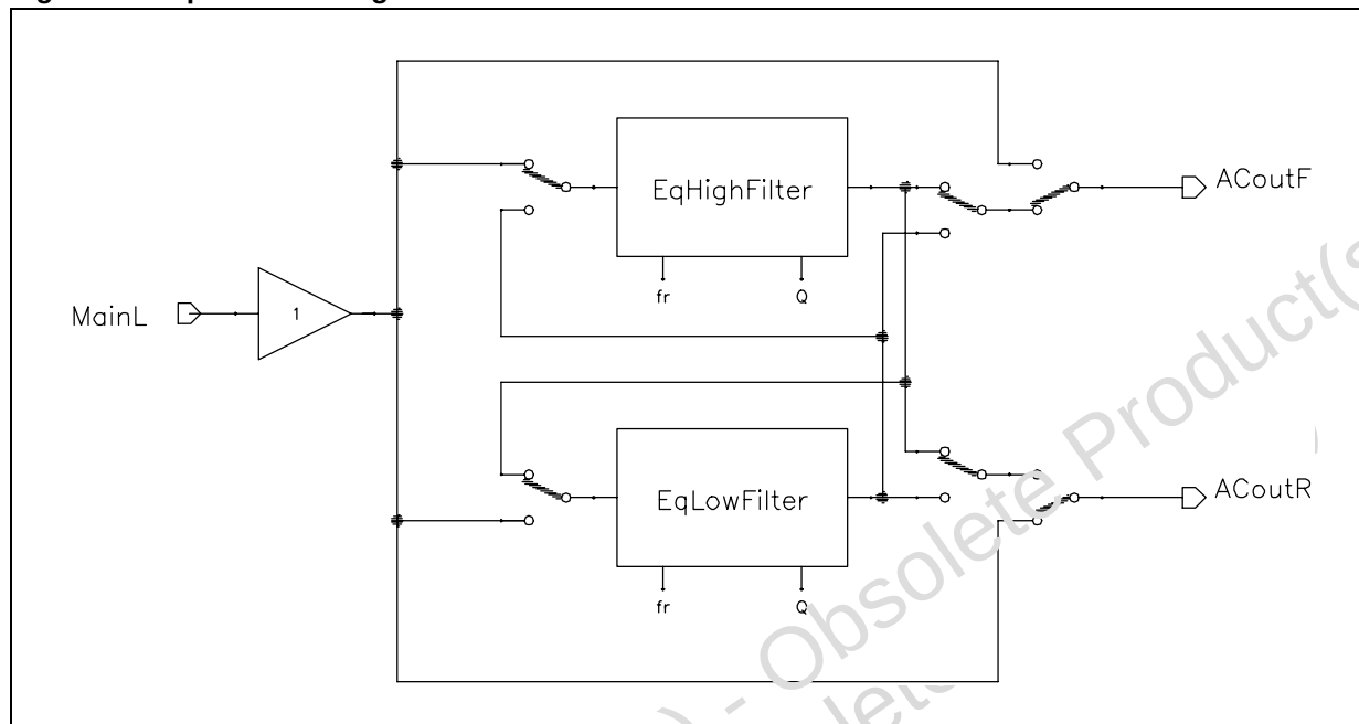
Figure 17. Equalizer Configuration
