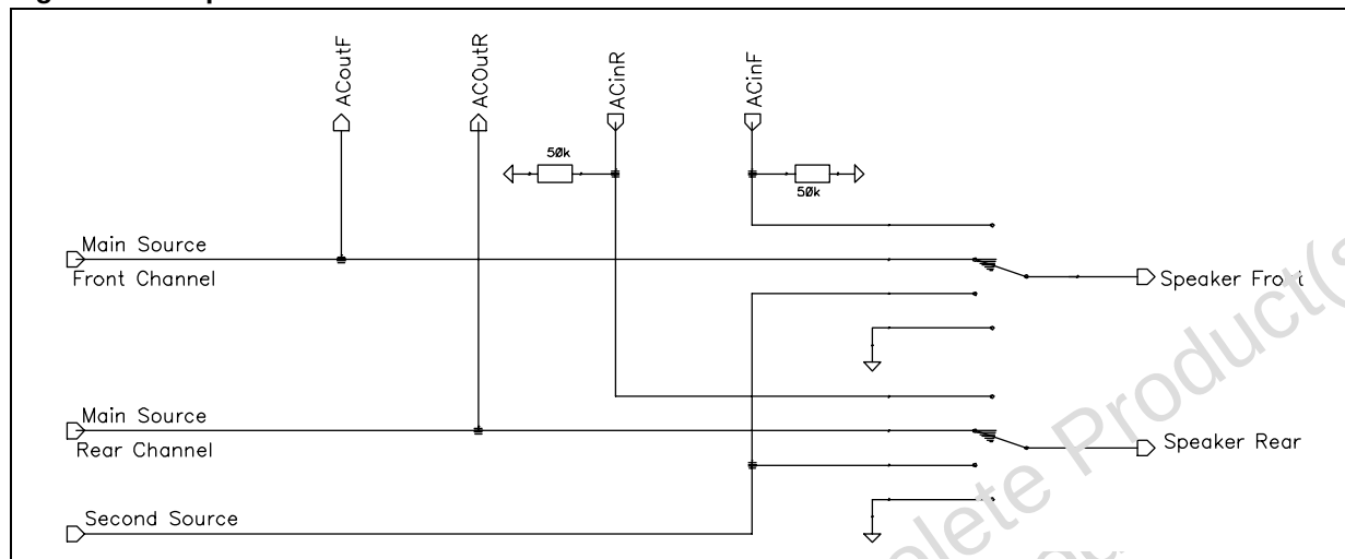
Figure 23. Output Selector
