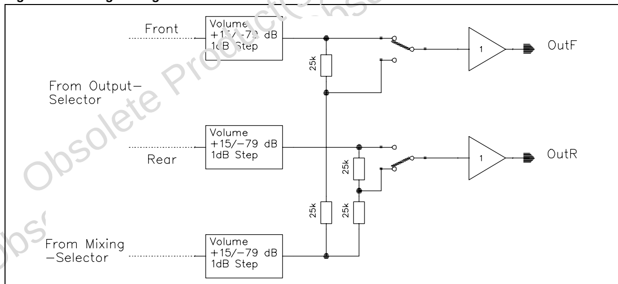
Figure 24. Mixing Configuration
