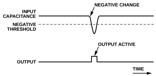
Figure 13. Negative Threshold Mode Indicates Negative Change in Input Capacitance
