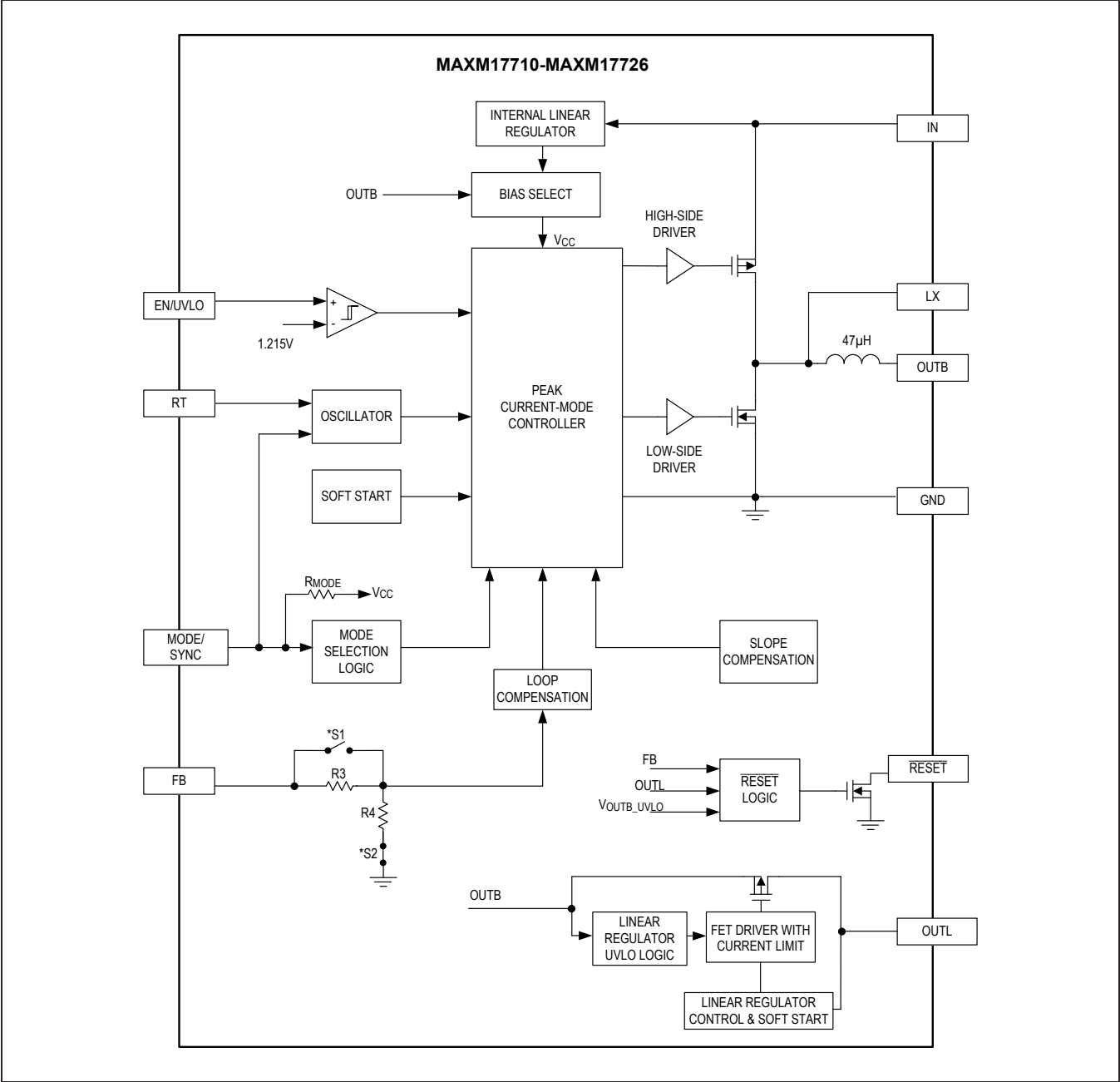
Functional Diagram
