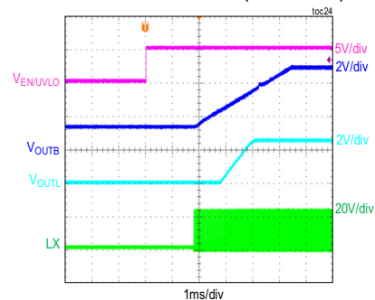
MAXM17724 STARTUP THROUGH ENABLE (1.5V PREBIAS)
