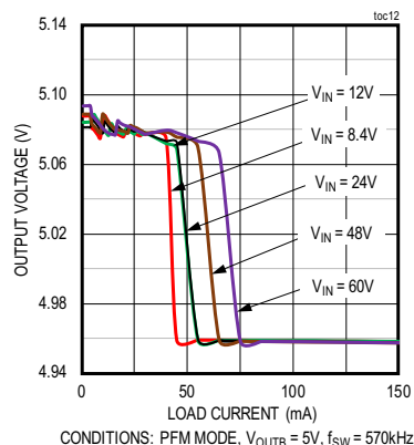
MAXM17715-MAXM17720, MAXM17721-MAXM17726 OUTPUT VOLTAGE vs. LOAD CURRENT
