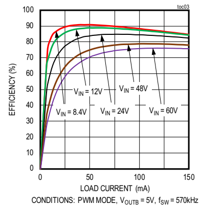
MAXM17715-MAXM17720, MAXM17721-MAXM17726 EFFICIENCY vs. LOAD CURRENT
