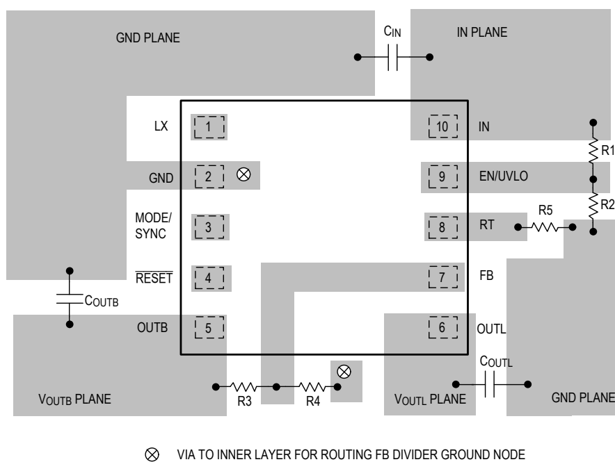
Figure 4. Adjustable Output Layout Guidelines
