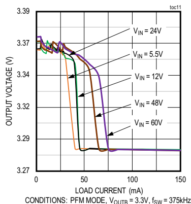
MAXM17710-MAXM17714, MAXM17721-MAXM17726 OUTPUT VOLTAGE vs. LOAD CURRENT
