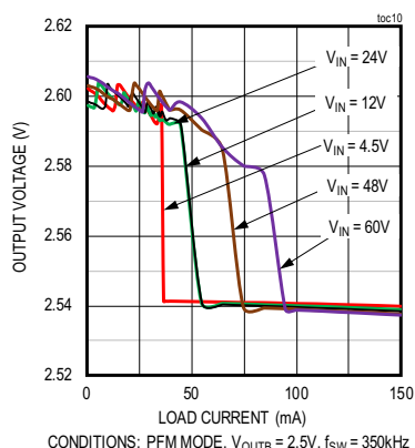
MAXM17721-MAXM17726 OUTPUT VOLTAGE vs. LOAD CURRENT
