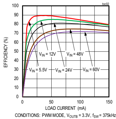
MAXM17710-MAXM17714, MAXM17721-MAXM17726 EFFICIENCY vs. LOAD CURRENT
