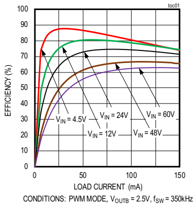
MAXM17721-MAXM17726 EFFICIENCY vs. LOAD CURRENT
