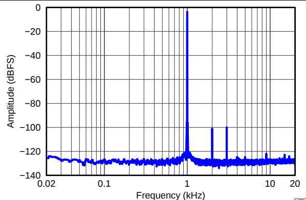
Figure 8. ADC Single Ended Input to ADC Fft at -3 DBR vs Frequency
