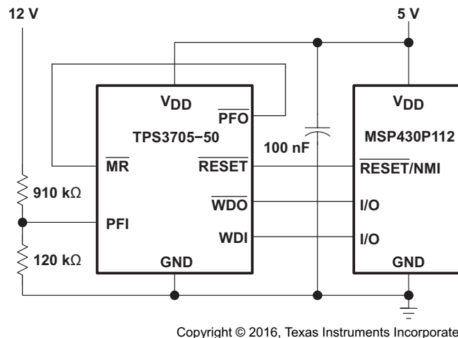
Figure 9. Typical MSP430 Application
