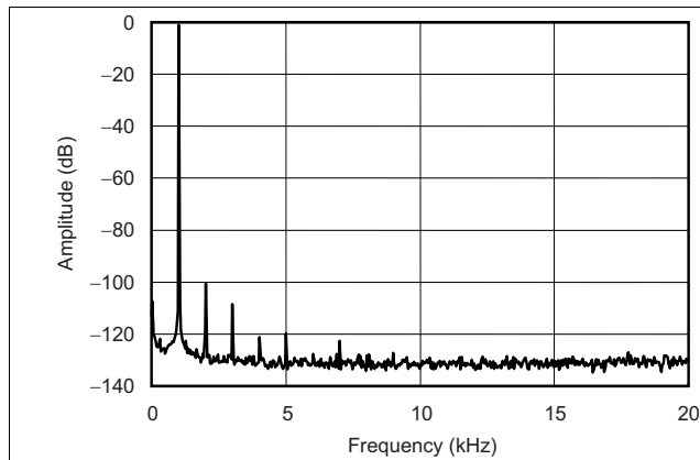
Figure 9. Output Spectrum
