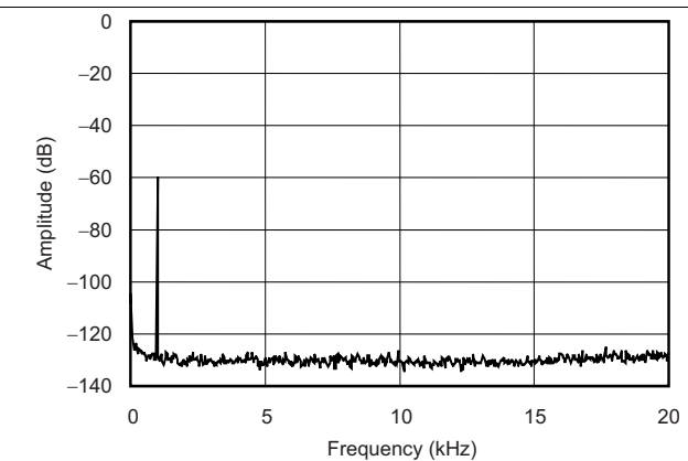
Figure 10. Output Spectrum
