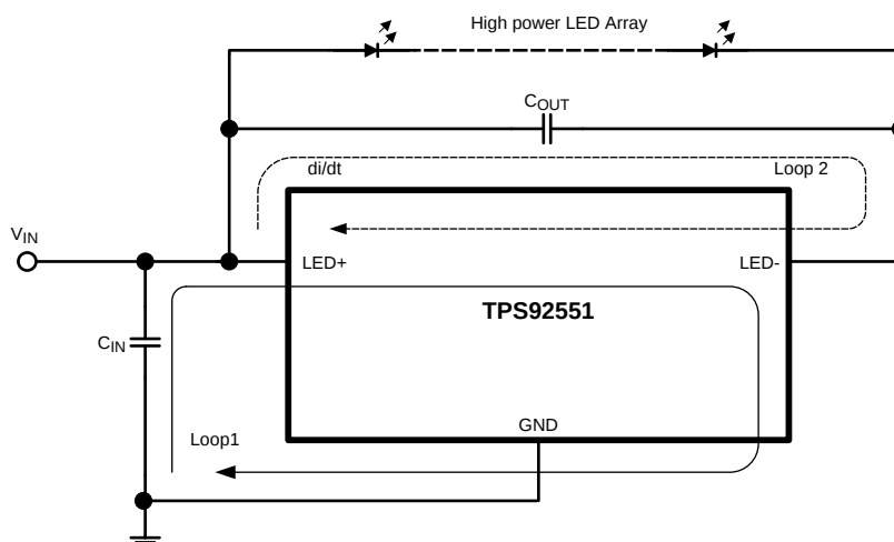
Figure 36. Current Loops
