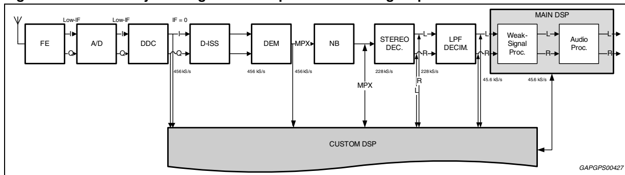
Figure 4. Secondary DSP signal access points in main signal path
