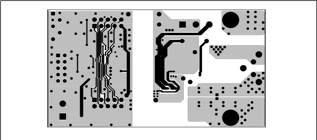
Figure 4. STGAP1AS – layout (bottom layer)
