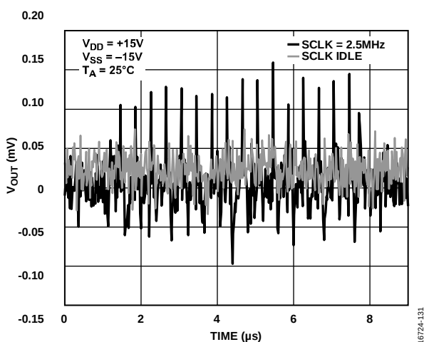
Figure 29. Digital Feedthrough
