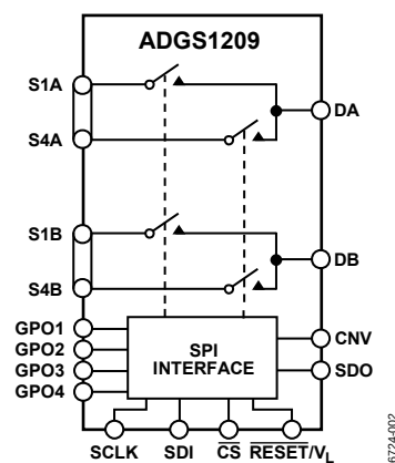
Figure 2. ADGS1209 Functional Block Diagram
