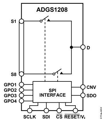
Figure 1. ADGS1208 Functional Block Diagram
