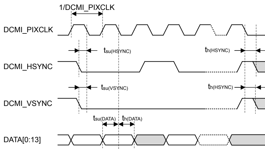
Figure 51. DCMI timing diagram
