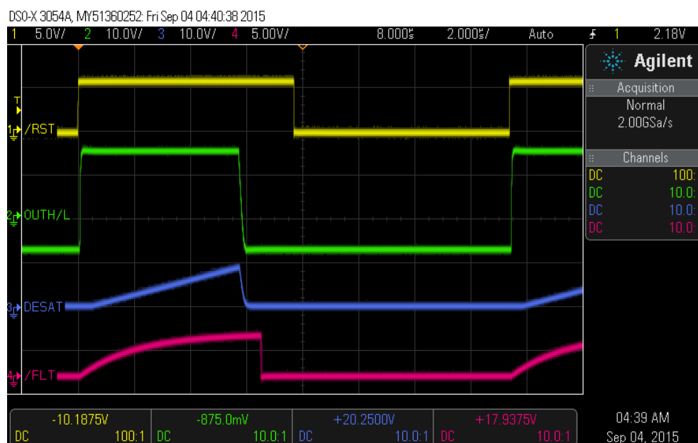
Figure 8. ISO5852S EVM OUTH/L, DESAT, \overline{\text{FLT}} , and \overline{\text{RST}} With Bipolar Output Supply
