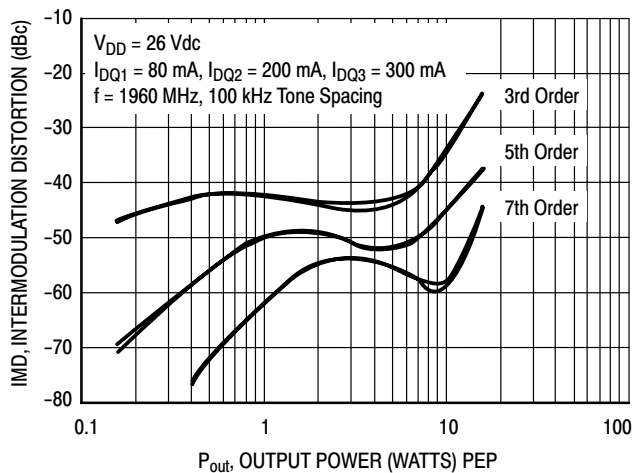
Figure 7. Intermodulation Distortion Products versus Output Power @ 1960 MHz
