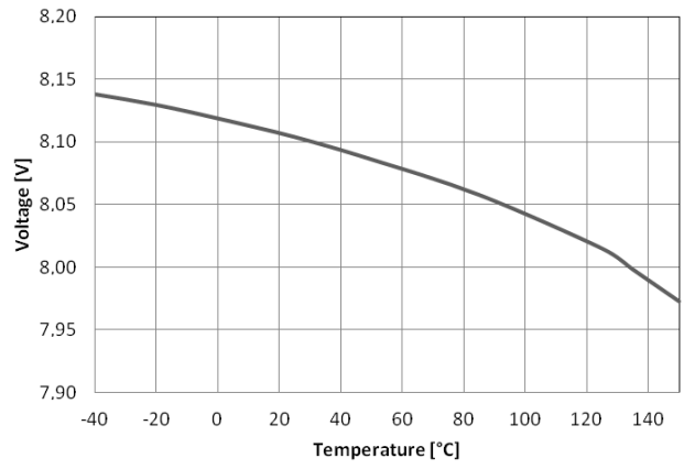
Figure 6. V CCOff vs. Temperature
