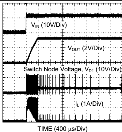
Figure 28. Power Up
