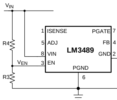
Figure 24. Adjustable UVLO
