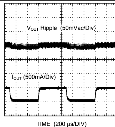
Figure 29. Load Transient
