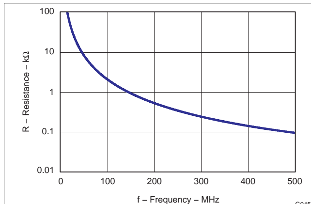
Figure 46. ADC Analog Input Resistance (Rin) Across Frequency
