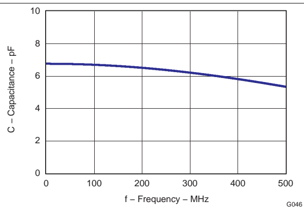
Figure 47. ADC Analog Input Capacitance (Cin) Across Frequency
