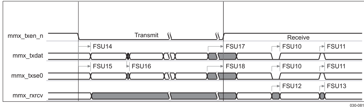
Figure 6-48. Low-/Full-Speed USB Bidirectional Standard 4-pin Mode
