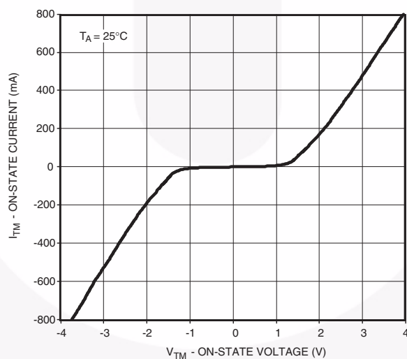
Fig. 9 On-State Characteristics
