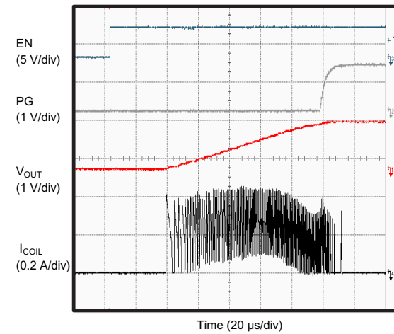
Figure 29. Start Up (Without Load)
