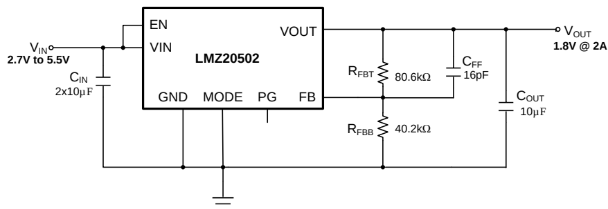
Figure 16. LMZ20502 Typical Application V_{OUT} = 1.8 V
