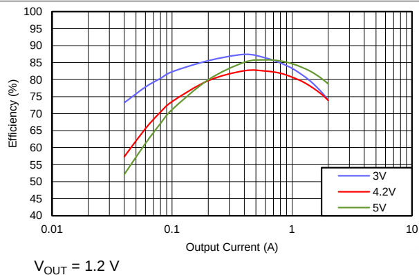
Figure 26. Efficiency
