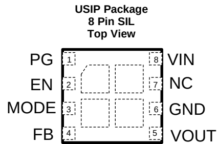
Pin Functions
