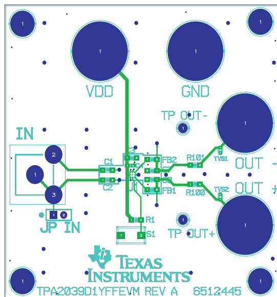
Figure 1. Top Layer
