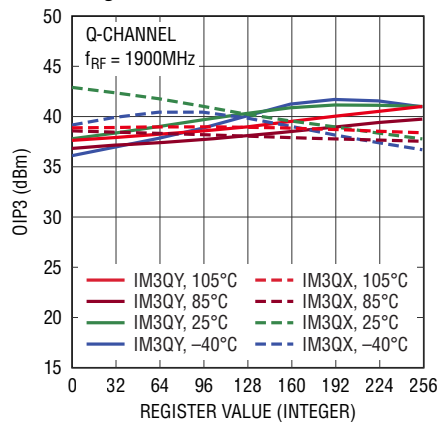
OIP3 vs Temperature ( T_C ) and Register Value, Q-Channel
