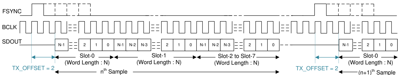
Figure 18. TDM Mode Protocol Timing (TX_OFFSET = 2)
