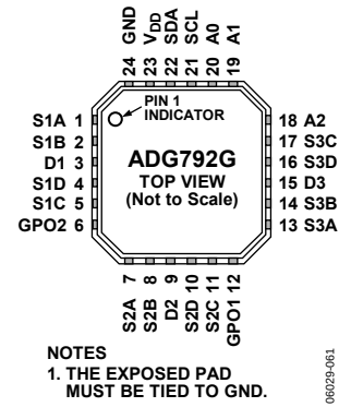
Figure 4. ADG792G Pin Configuration
