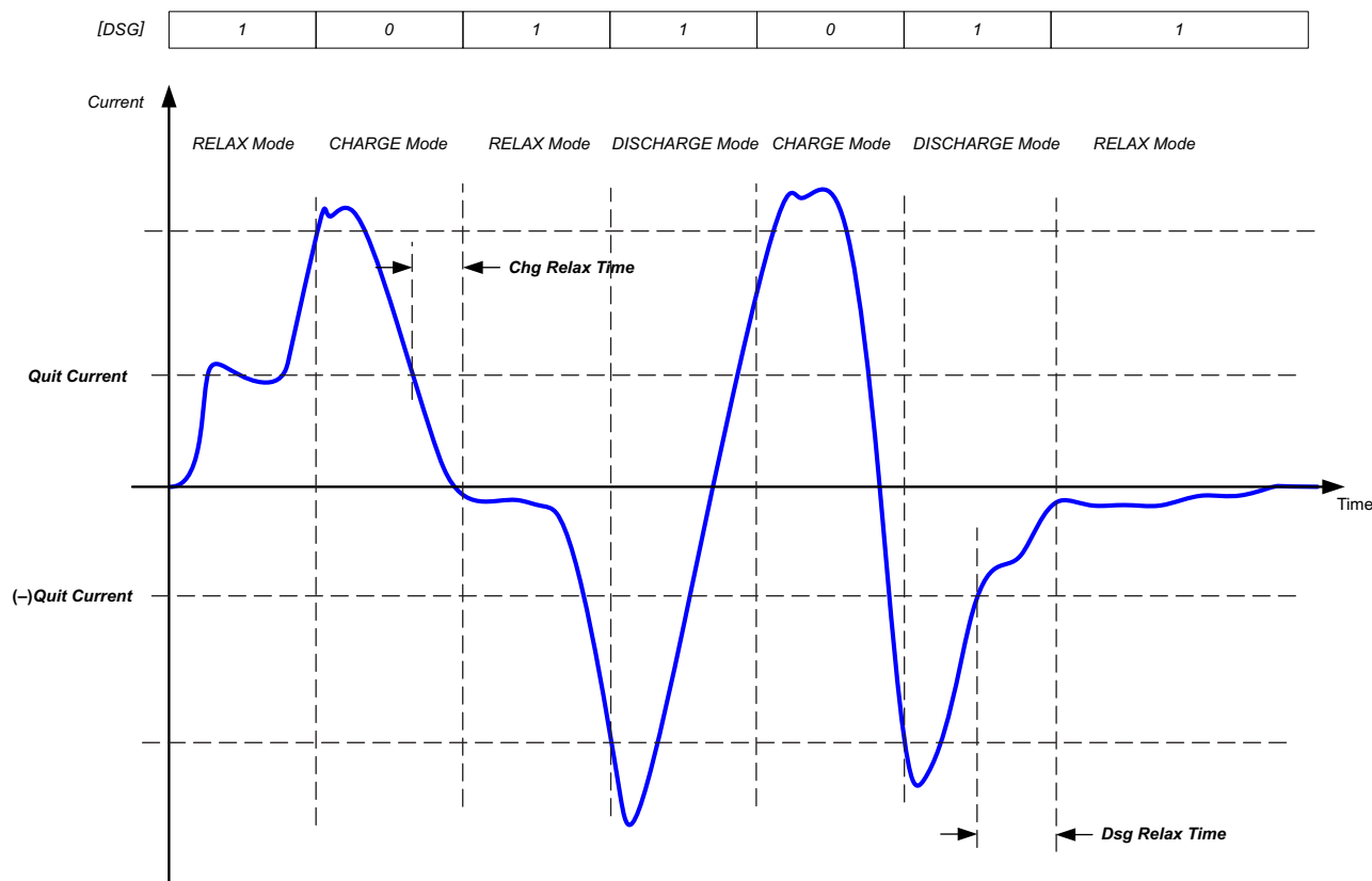
Figure 6-2. Gas Gauge Operating Mode Example
