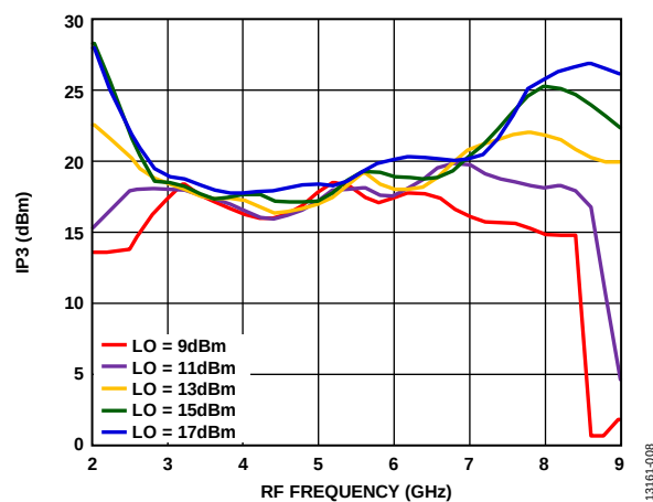
Figure 15. Input IP3 vs. RF Frequency at Various LO Drives
