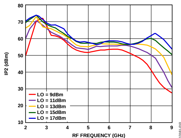
Figure 16. Input IP2 vs. RF Frequency at Various LO Drives
