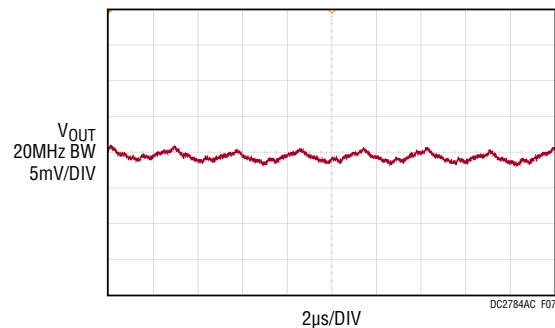
Figure 7. Output Voltage Ripple at V_{IN} = 12V , V_{OUT} = 1.0V , I_{OUT} = 400A
