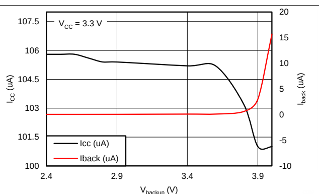
Figure 3. Current Consumption vs Backup Supply Voltage
