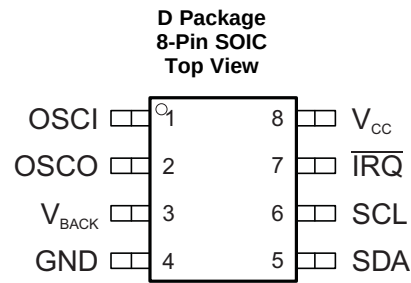
Pin Functions
