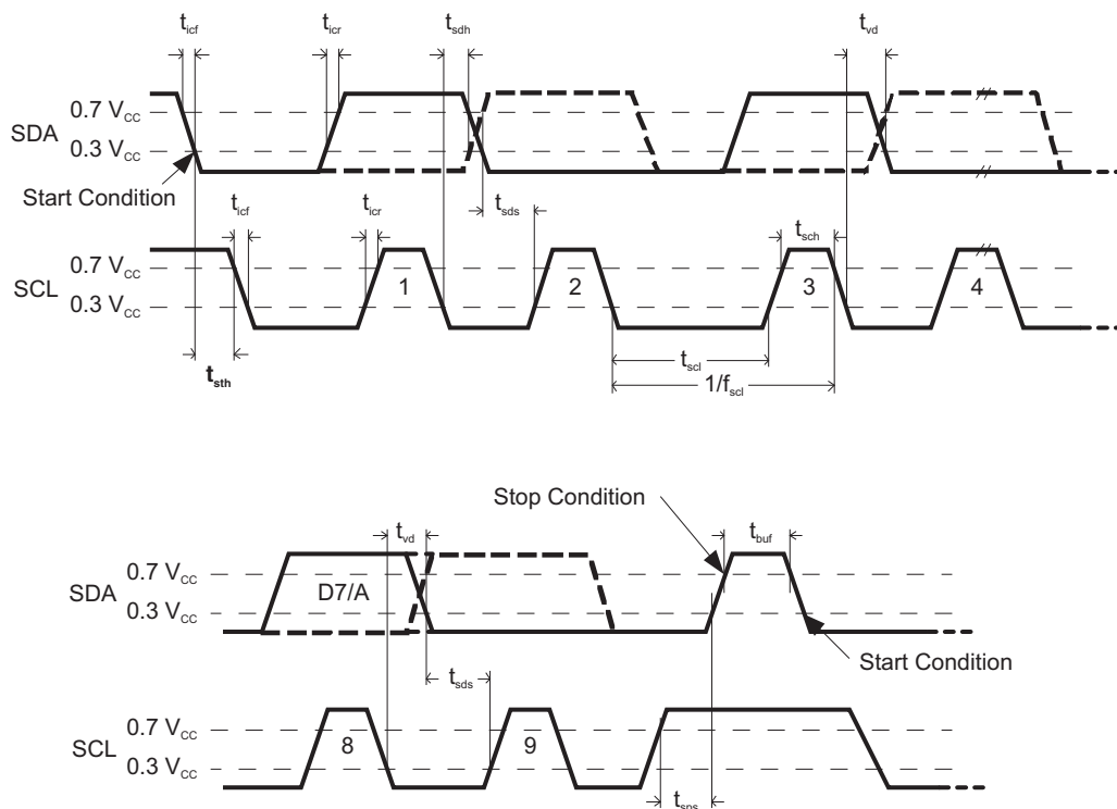
Figure 1. I²C Timing Diagram
