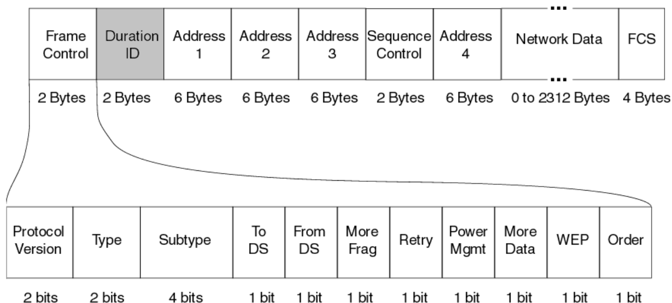
Figure 16-1. 802.11 Frame Structure
