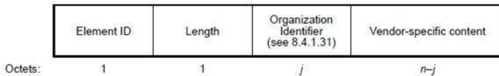
Figure 8-189—Vendor Specific element format
