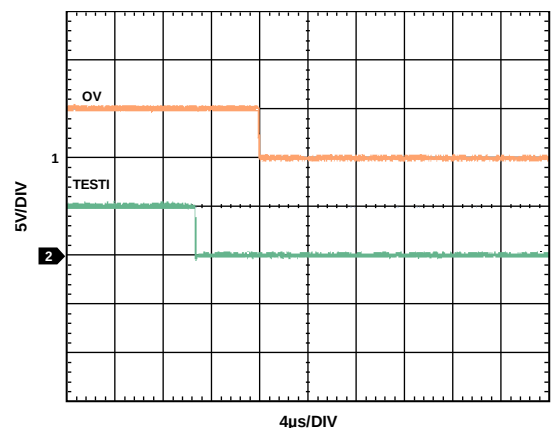
Figure 38. TESTI Edge and AVOUTxx, Self-Test Fails (Enlarged)
