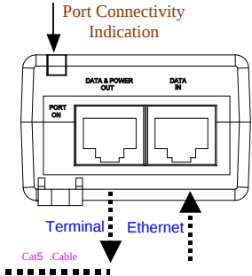
Figure 1: Connecting the PD-9001GR
