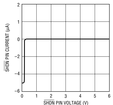
\overline{SHDN} Pin Current
