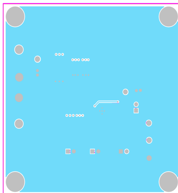
Figure 5. Middle Layer 2
