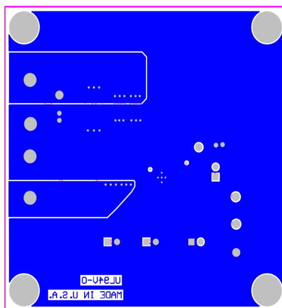
Figure 6. Bottom Layer
