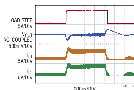
Load Step Pulse-Skipping Mode
